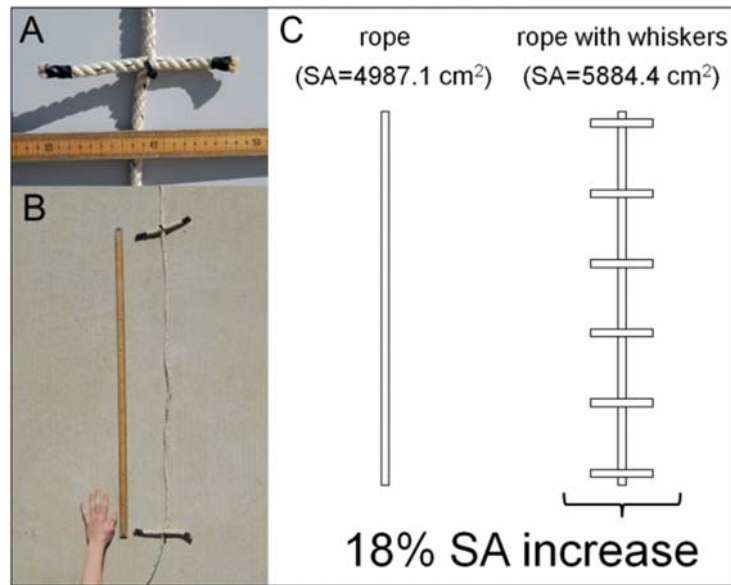
Figure 1. Experimental rope with 20cm-long “whisker” add-on devices that increase standard rope surface areas (SA) by 18% (Kot et al., in submission).
